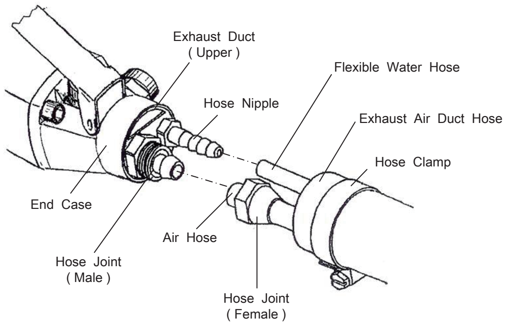
Figure 6 Connections of Hoses
