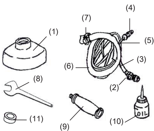
Figure 3 Standard Accessories
